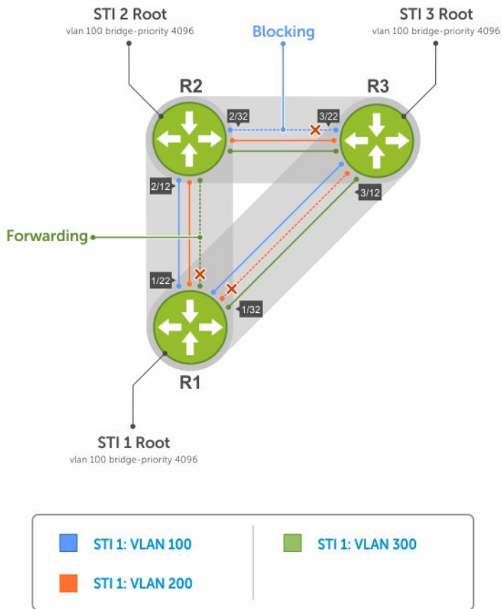
Figure 97. Load Balancing with PVST+
